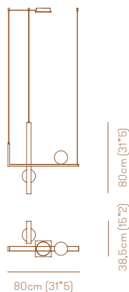
3x12W strip LED 24V 1250lm 2700°K Dimm. + 2x5W G9 LED 350lm 2700°K Dimm.
