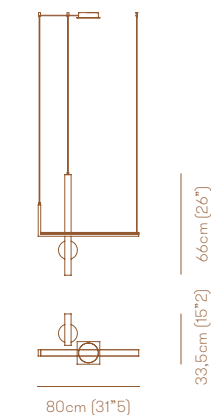
1x12W strip LED 24V 1250lm 2700°K Dimm. + 2x5W G9 LED 350lm 2700°K Dimm.
