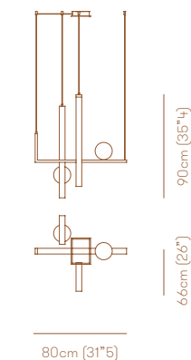
1x12W strip LED 24V 1250lm 2700°K Dimm. + 2x5W G9 LED 350lm 2700°K Dimm.
