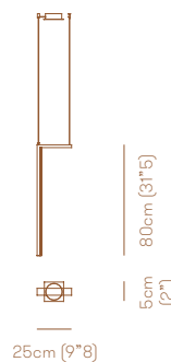
1x12W strip LED 24V 1250lm 2700°K Dimm. + 1x5W G9 LED 350lm 2700°K Dimm.
