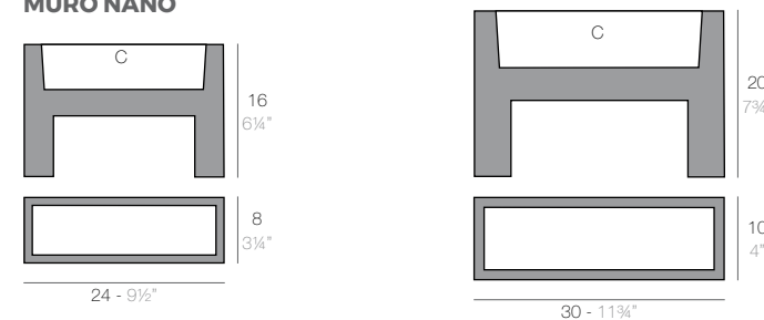
MURO NANO 24 x 8 x 16 cm WALL NANO 9½" x 3¼" x 6¼" MURO NANO 30 x 10 x 20 cm WALL NANO 11¾" x 4" x 7¾"
