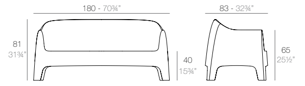
SOLID Sofa SOLID Sofá Ref: 55022
