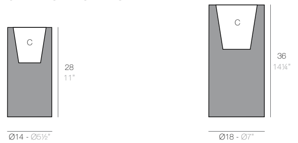
CILINDRO ALTO NANO Ø14 cm HIGH CYLINDER NANO Ø5½" CILINDRO ALTO NANO Ø18 cm HIGH CYLINDER NANO Ø7"
