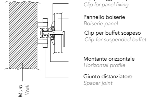
DETAIL 3 a) Aggancio a muro Wall mounting
